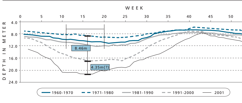
FIGURE 4 Average groundwater depth from the surface
