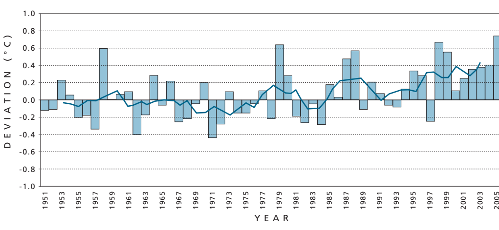
FIGURE 7 Deviation of yearly average minimum temperature from normal (1961 – 1990) with five-year moving average over Bangladesh
